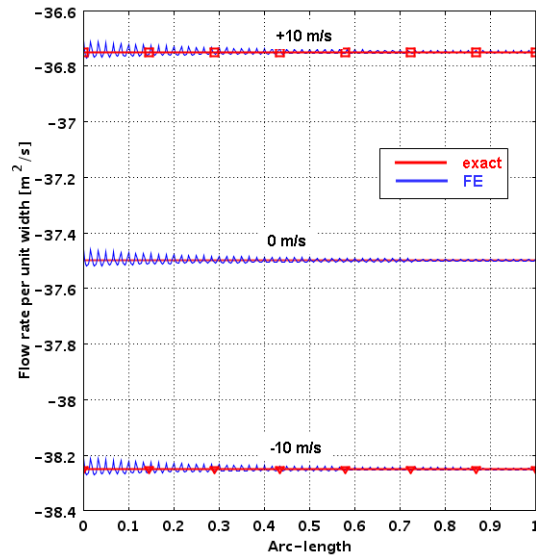
Figure 3. Variation of volumetric flow rate for plunger velocities of 0, -10 and +10 m/s. The arc length is defined from bottom to top of plunger.
